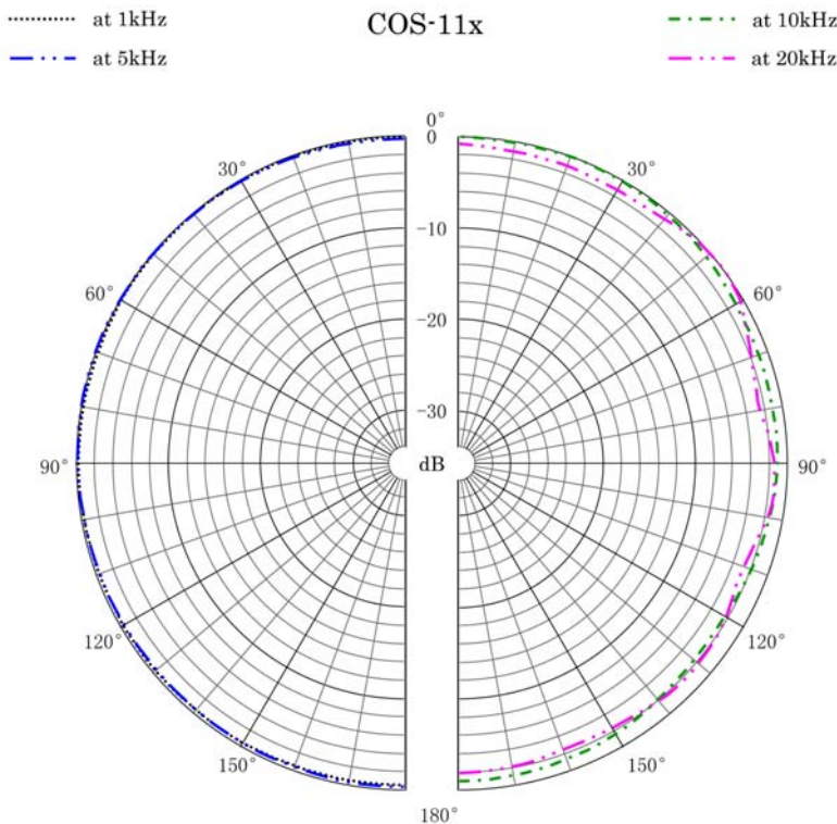
Polar Pattern
